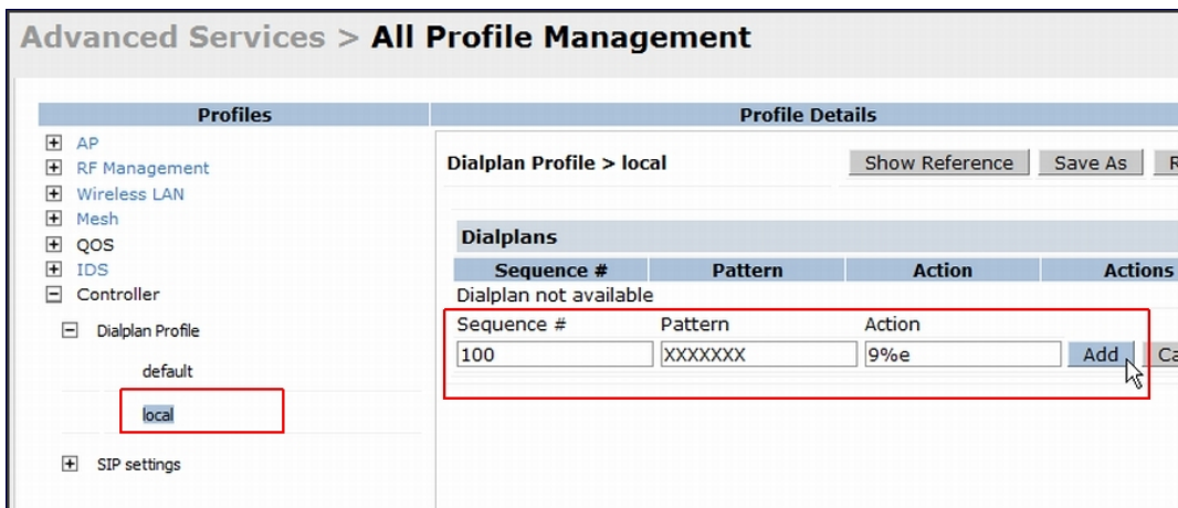
Figure 168 Dialplan Details
