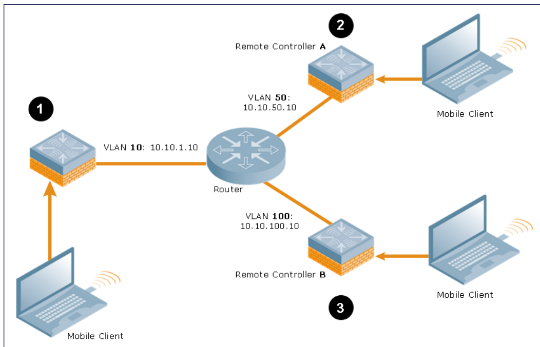
Figure 64 Inter-switch Mobility
