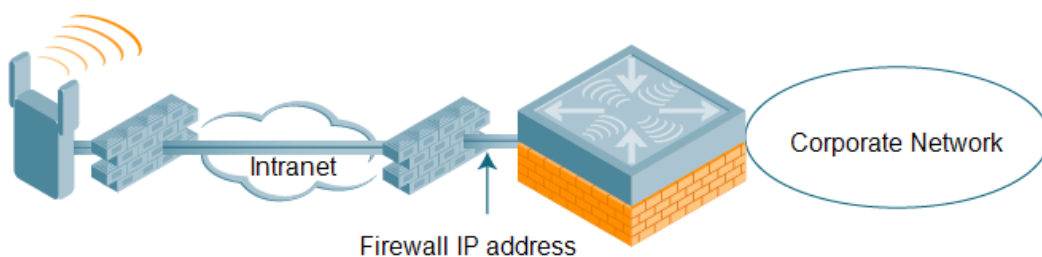
Figure 67 Remote AP with Switch Behind Firewall
