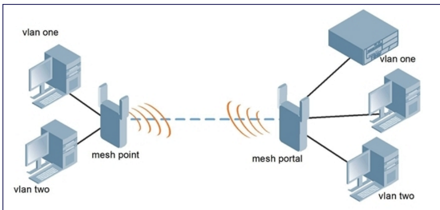
Figure 49 Sample Point-to-Point Deployment
