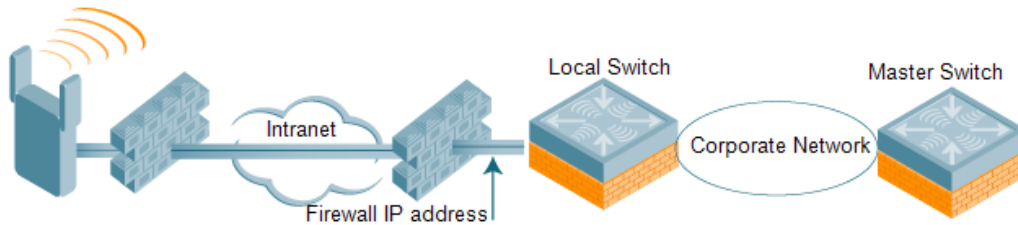
Figure 68 Remote AP in a Multi-Switch Environment
