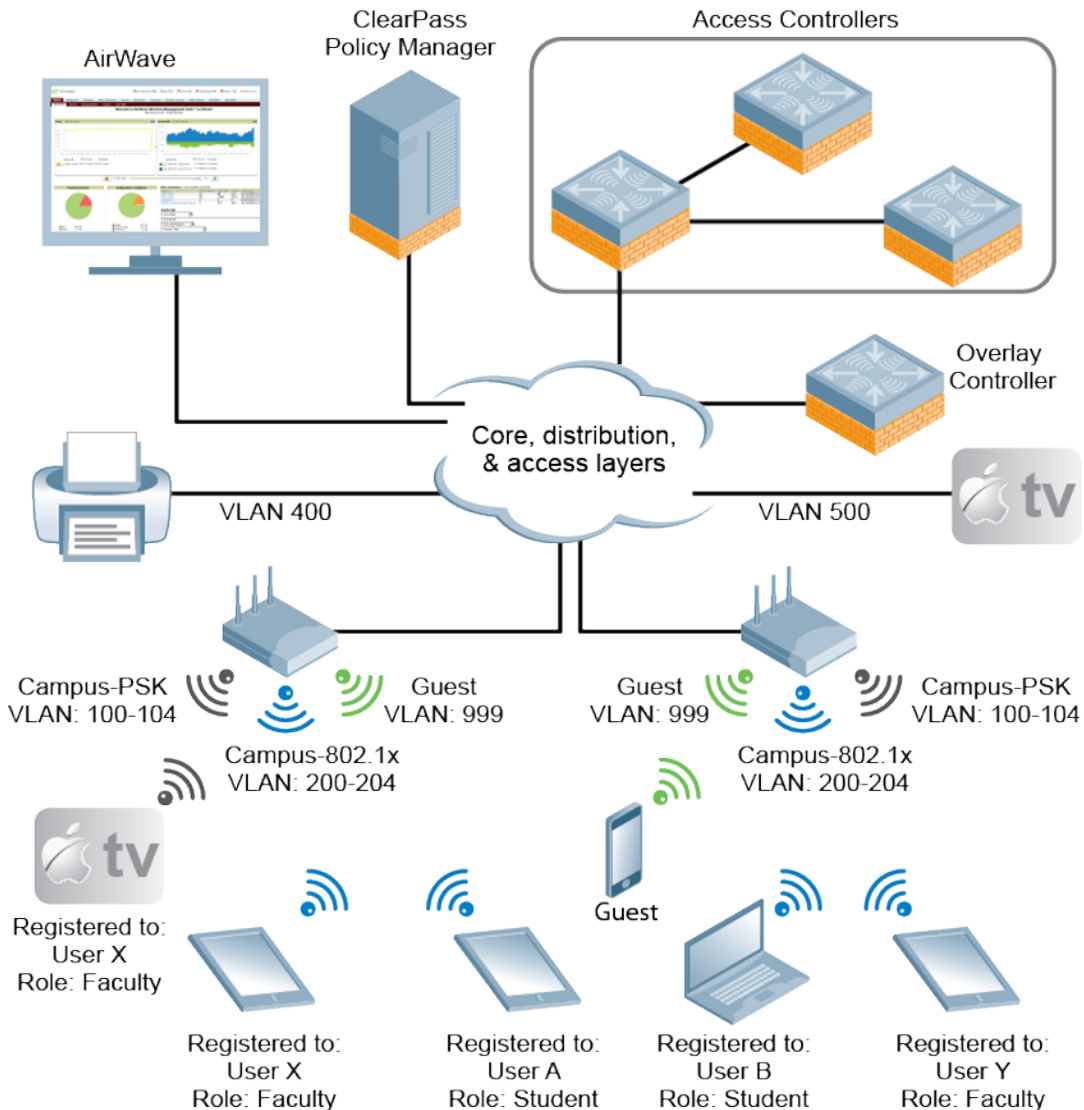
Figure 178 Overlay AirGroup Network Topology
