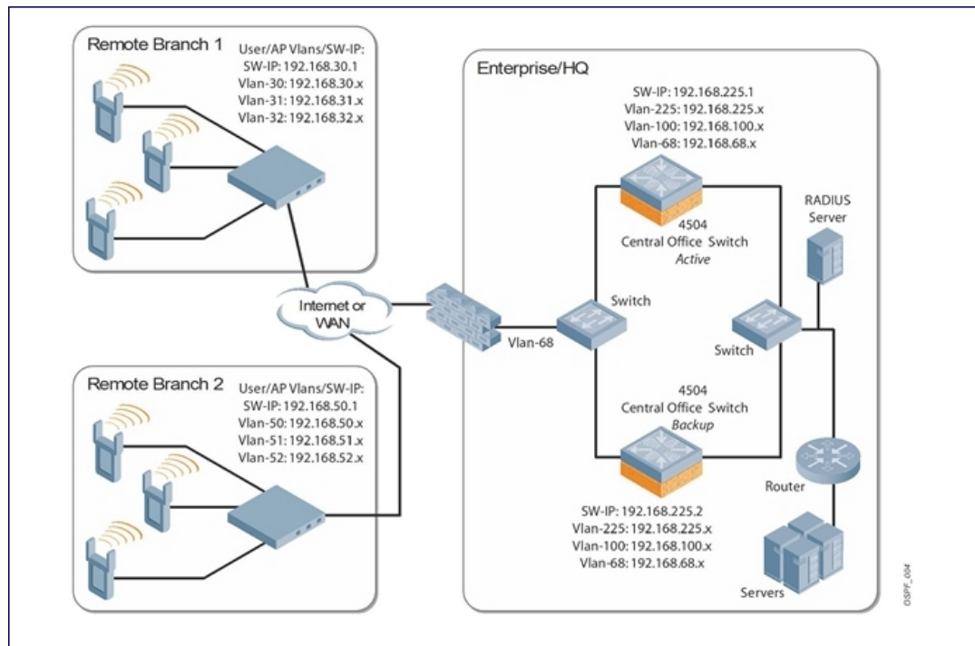
Figure 27 Sample OSPF Topology
