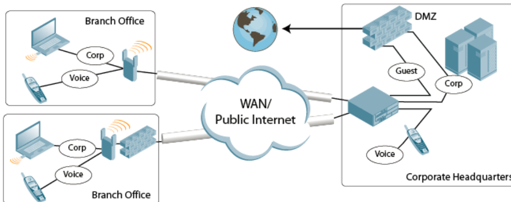
Figure 72 Remote AP with Single Switch
