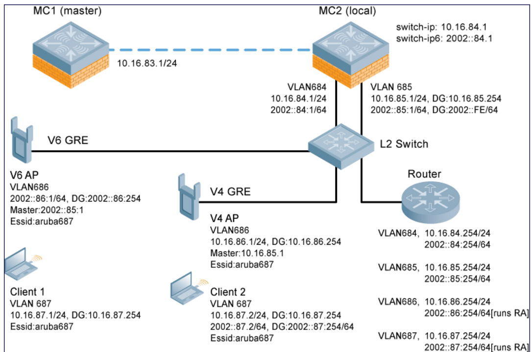
Figure 20 IPv6 Topology
