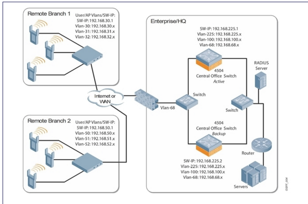
Figure 204 4306 Series Sample Topology
