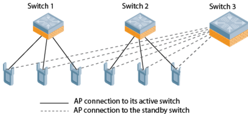
Figure 57 1:1 Active/Standby Deployment
