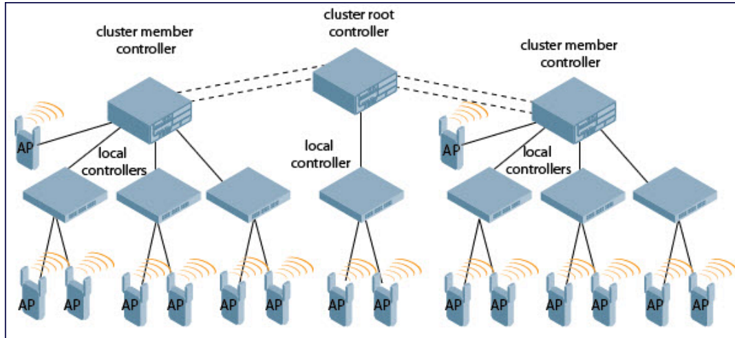
Figure 7 A Cluster of Master Switches using Control Plane Security
