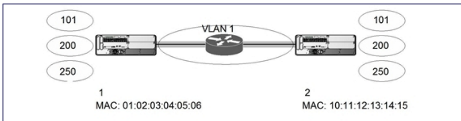
Figure 144 Switch-to-Switch xSec Example
