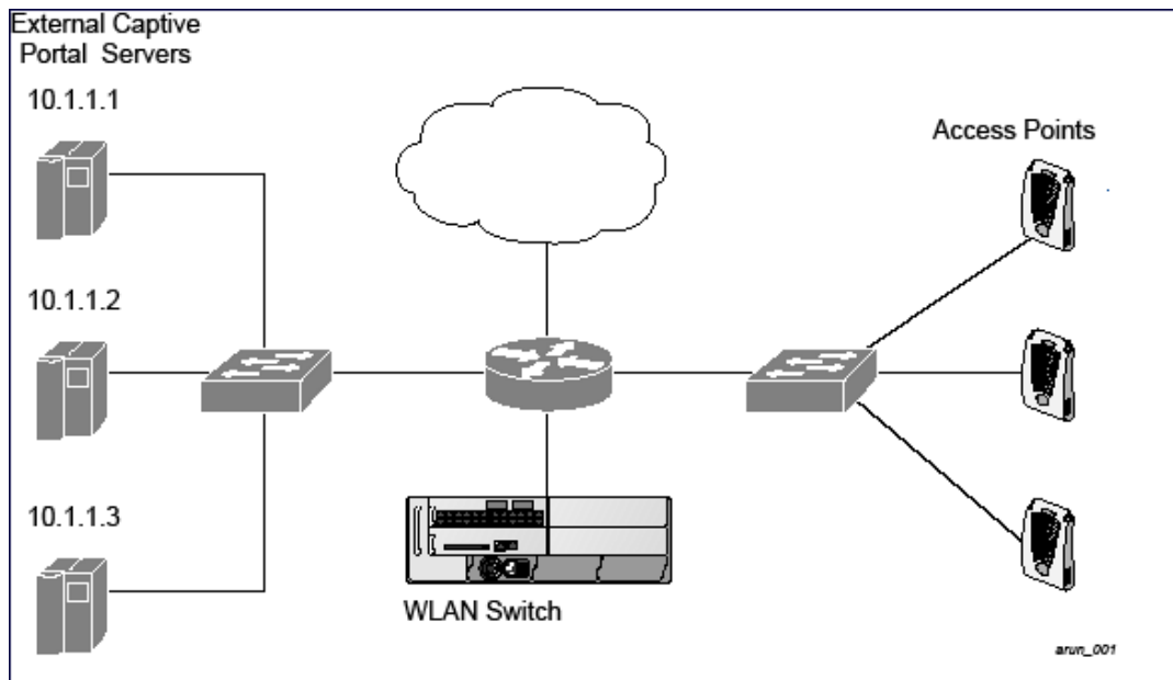
Figure 211 Example NAT-Mode Topology
