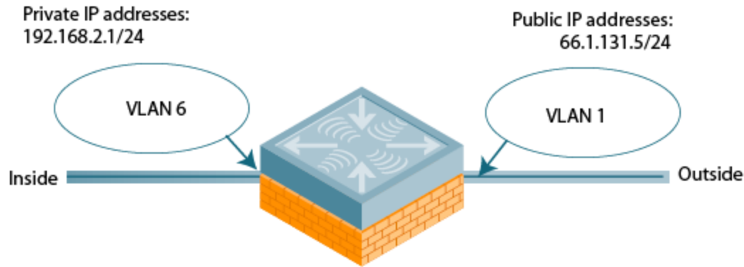
Figure 18 Example: Source NAT using Switch IP Address
