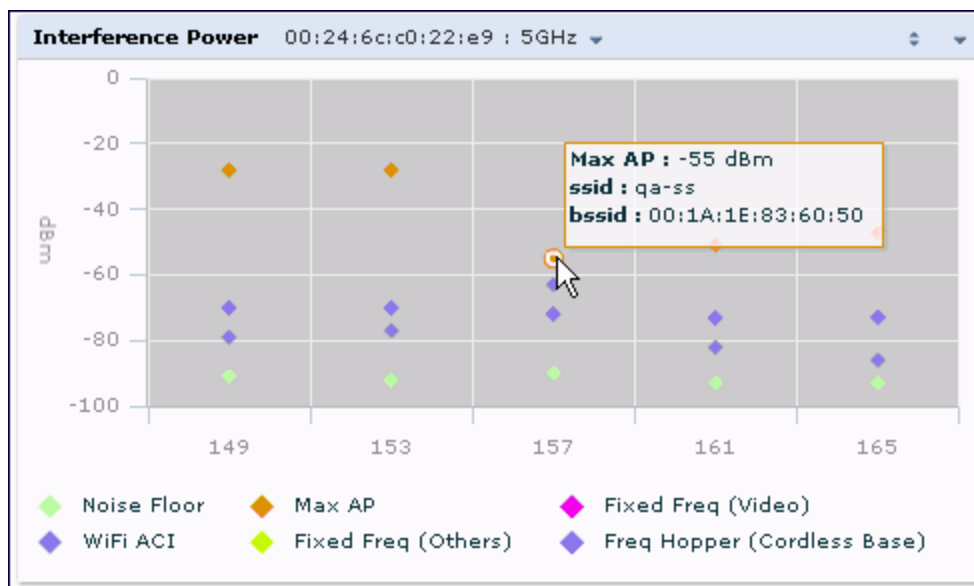
Figure 113 Interference Power
