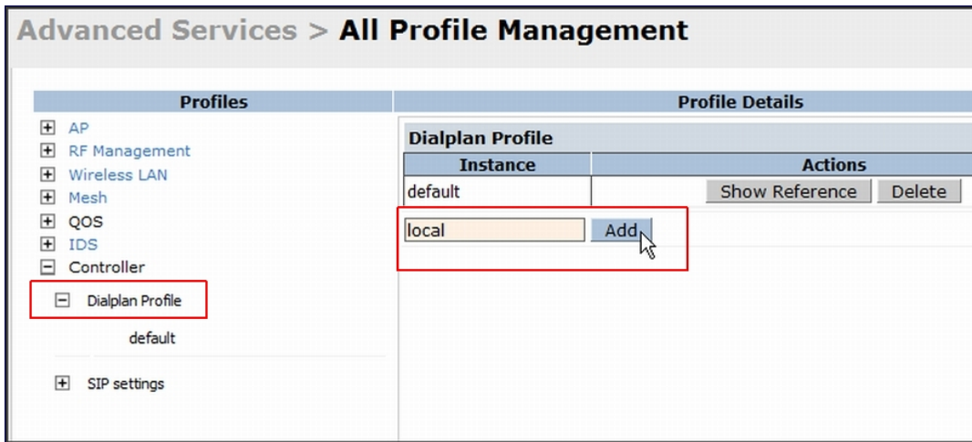
Figure 167 Dialplan Profile
