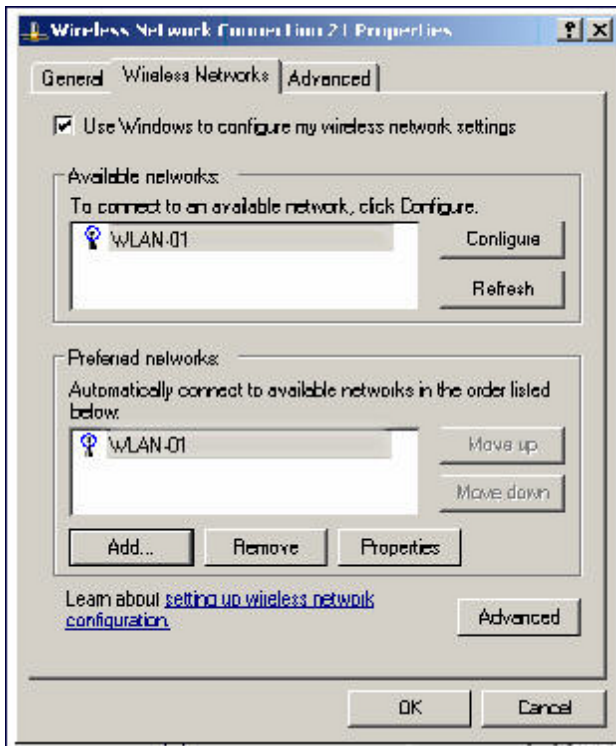
Figure 227 Wireless Networks
