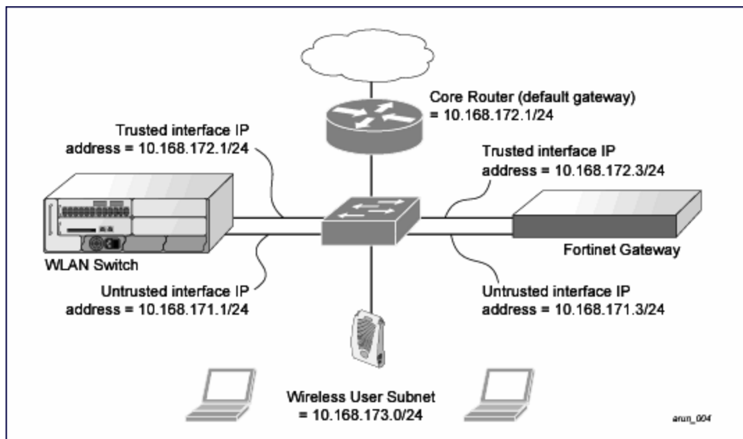
Figure 210 Example Route-Mode Topology
